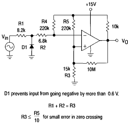
Figure 9. Zero Crossing Detector (Single Supply)
